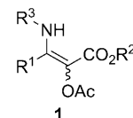
Figure 1. \alpha -Acetoxy \beta -enamino esters 1 that were subjected to hydrosilylation in this study.
